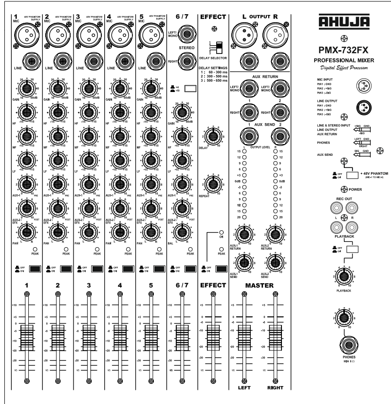
TOP PANEL
